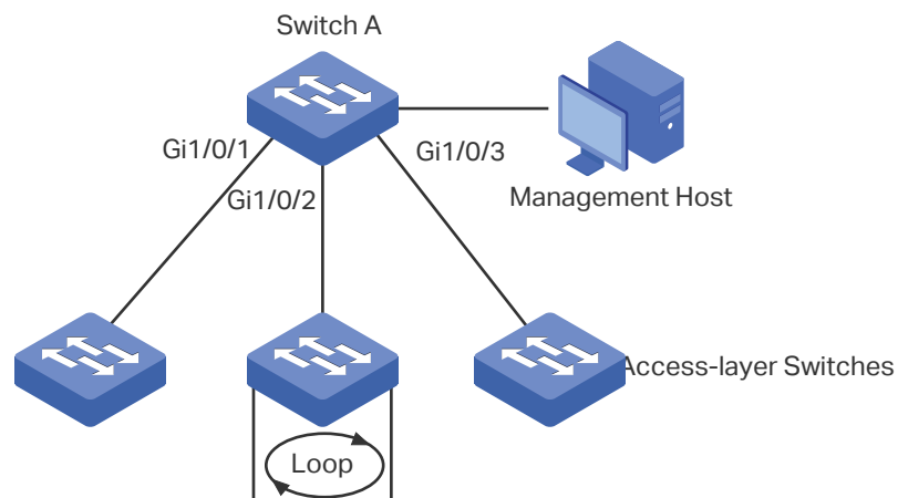
Figure 7-8 Network Topology
