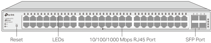
Figure 1-5 Front Panel of T1600G-52TS (TL-SG2452)
