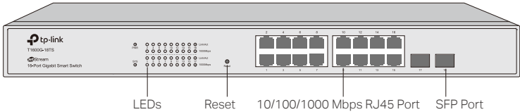
Figure 1-3 Front Panel of T1600G-18TS (TL-SG2216)
