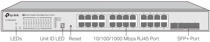
Figure 1-7 Front Panel of T1700G-28TQ
