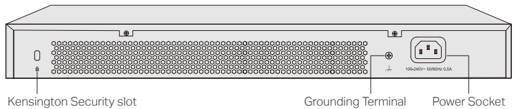
Figure 1-11 Rear Panel
