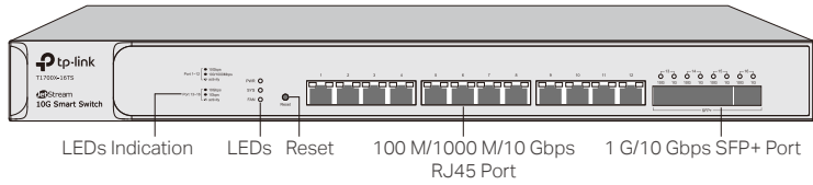
Figure 1-8 Front Panel of T1700X-16TS
