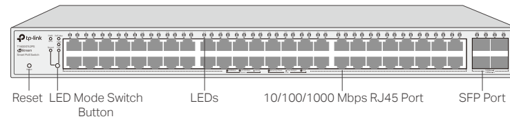
Figure 1-6 Front Panel of T1600G-52PS (TL-SG2452P)
