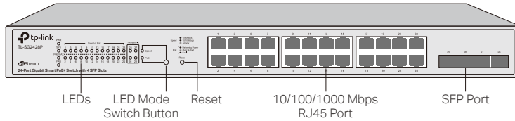
Figure 1-10 Front Panel of TL-SG2428P
